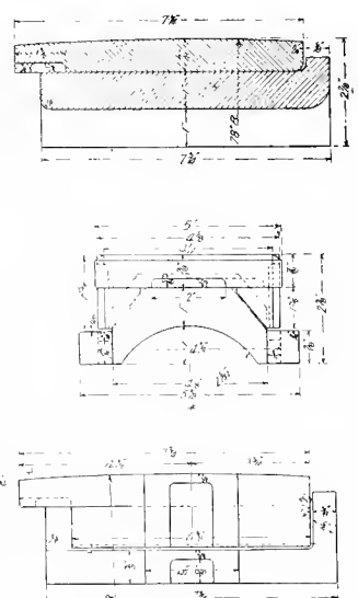
Figs. 5416-5418. WEDGE AND BEARING.
